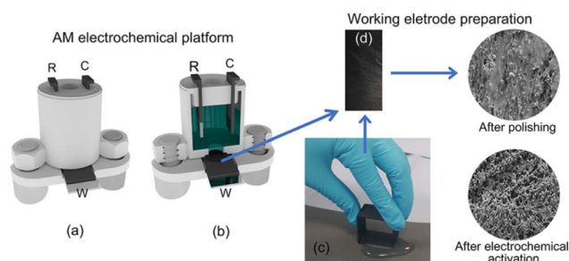
Fig. 2 Schematic representation of an efficient and commonly employed pretreatment performed on a CB/PLA 3D printed electrode. 29 Copyright, American Chemical Society.
