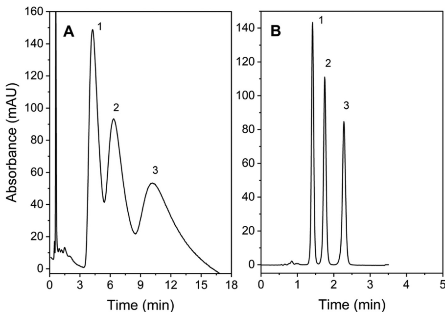
Fig. 4 Chromatograms illustrating the separation of model compounds in columns with p -PDA-derived phases containing (A) 13 rings per nm 2 and (B) 4 rings per nm 2 on 5 μm-Kinetex® core-shell silica particles (columns dimensions: 50 mm length, 2.1 mm i.d.). A mobile phase of 50/50 acetonitrile/water was used at a flow rate of 0.2 mL min -1 ; UV detection was performed at 210 nm. Compounds: (1) toluene, (2) ethylbenzene, and (3) propylbenzene (100 μg mL -1 each, 1 μL injection).
