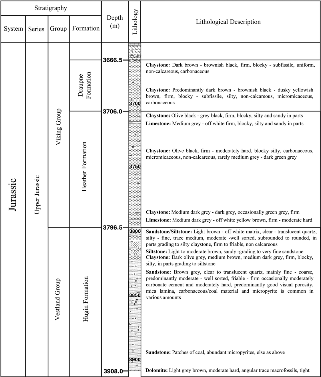
Fig. 3 Stratigraphic column and facies description of the considered subsurface section. Adapted from Statoil. 41
