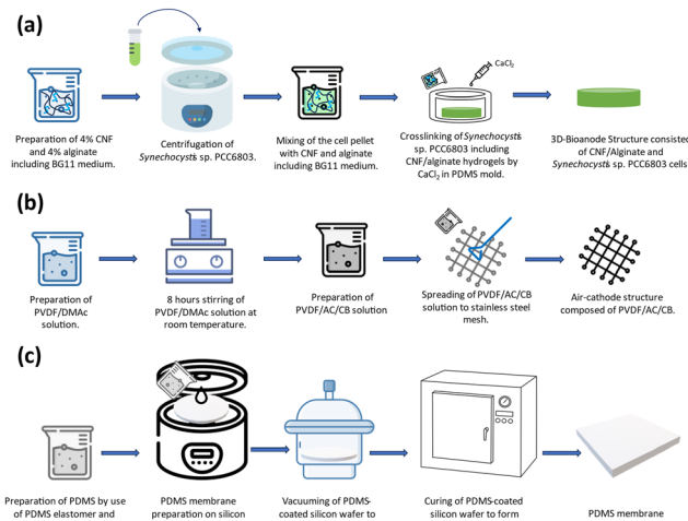
Fig. 2 The fabrication process of (a) 3D-Bioanode composed of CNF/alginate and Synechocystis sp. PCC 6803. (b) Air-cathode consisting of PVDF/AC/CB. (c) PDMS membrane.
