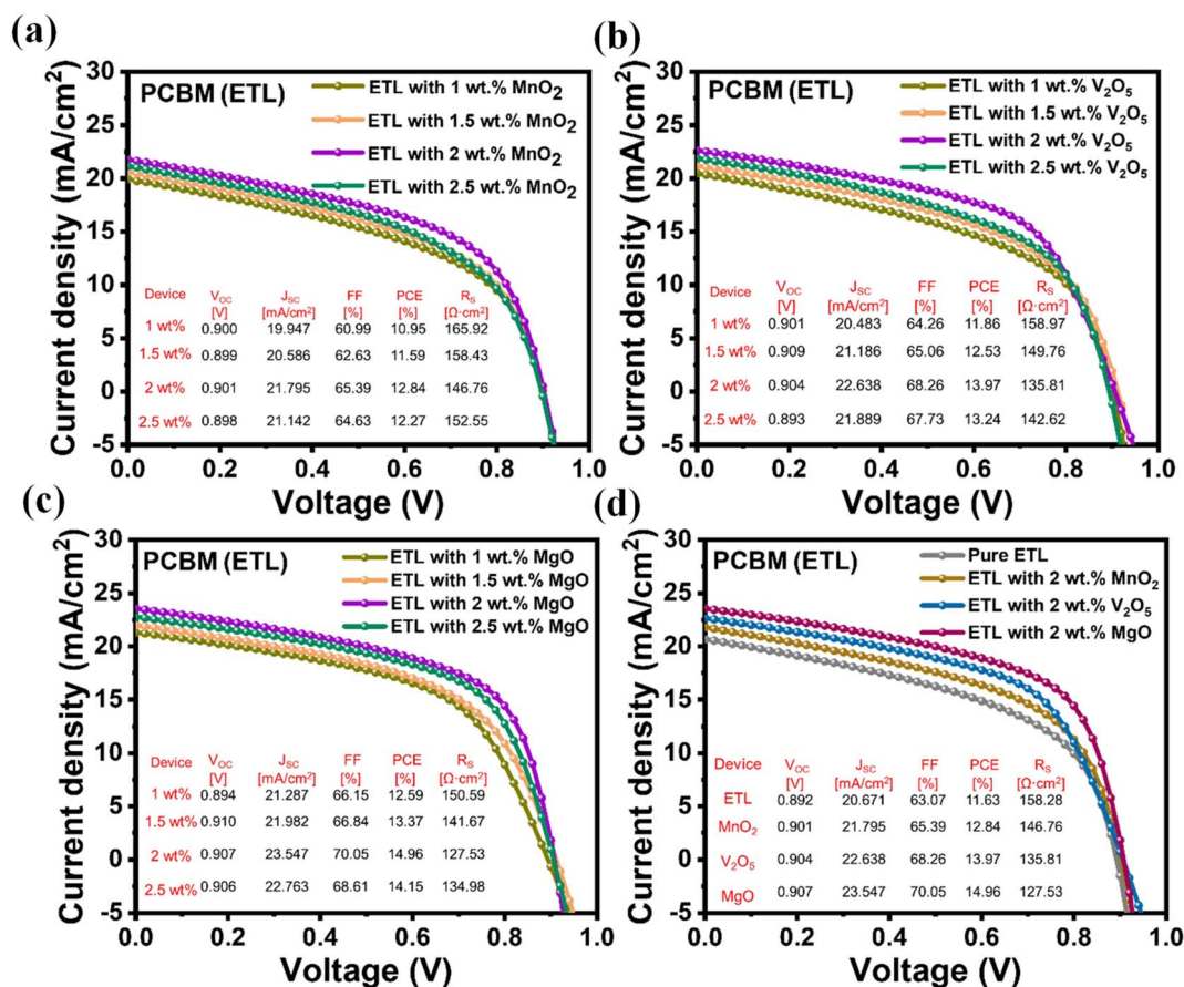
Fig. 7 J - V profiles for 1, 1.5, 2 and 2.5 wt% of (a) MnO 2 , (b) V 2 O 5 , and (c) MgO doped PCBM as ETLs. (d) J - V profiles for pure and optimized (2 wt%) V 2 O 5 , MnO 2 , and MgO hybrids doped ETL.
