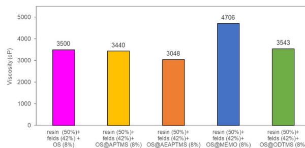
Fig. 4 Viscosity values for the mixtures resin/feldspar/OS@silanized (50/42/8 %w/w). All the measurements were performed in triplicate (Table S7†).
