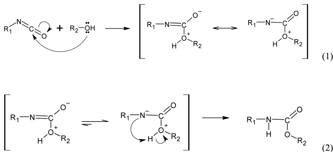
Fig. 12 Simplified reaction mechanism of urethane bonds formation from the reaction between isocyanate group ( \text{R1-N=C=O} ) and an alcohol ( \text{R2-OH} ), where R1 and R2 are carbon side chains.
