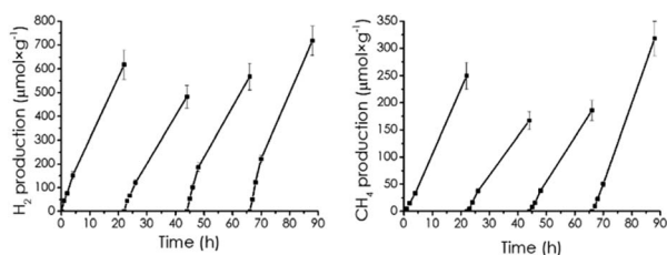
Fig. 5 Temporal evolution of hydrogen and methane production during photocatalytic irradiation of CD-1/mpC in four consecutive uses. Reaction conditions: acetonitrile 12 mL, H 2 O 4 mL, triethanol amine 4 mL, CD-1/mpC at 0.5 mg mL -1 , irradiation through quartz with the full output of a 300 W Xe lamp.
