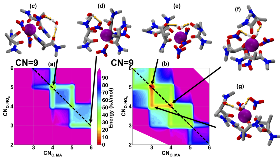
Fig. 4 Lu(III) solvation free energy landscapes in hexane from MD. x - and y -axis in (a) and (b) shows the CN_{O,MA} and CN_{O,NO_3} respectively. (a) shows the solvation free energy landscape when water at the out-sphere ( CN_{O,H_2O} = 0 ), while (b) shows the same when water at the inner-sphere ( CN_{O,H_2O} = 1 ). A total coordination number of 9 is denoted by the dashed black line. (c)–(g) shows representative molecular events labeled by black arrows on the map. Hydrocarbon tails of MA are replaced with the methyl group for simplicity. Yellow double arrows represent h-bond events.
