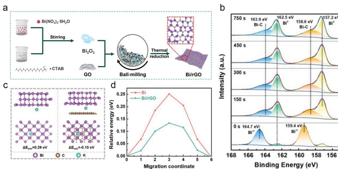
Fig. 7 (a) Schematic illustration for the preparation of Bi/rGO composites. (b) XPS Bi 4f spectra of Bi/rGO-2. (c) Potassium adsorption on the surface of Bi (102) and the interface of Bi/rGO. (d) The K^+ diffusion barrier energy in the Bi and Bi/rGO. Reproduced with permission. 51 Copyright 2024, Wiley-VCH.
