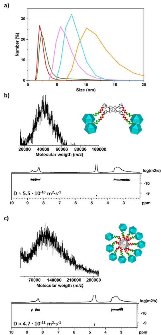
Fig. 3 (a) DLS spectra illustrating the differences in particle size (hydrodynamic-diameter) among the deprotected ( \text{N}_3 ) 1 -RhMOP (green), the deprotected (alkyne) 1 -RhMOP (red), the MOP-dimer (violet), the MOP-tetramer (cyan) and the MOP-satellite (orange). (b and c) MALDI-TOF spectra (top) and DOSY-NMR spectra (bottom) of MOP-tetramer (b) and MOP-satellite (c).
