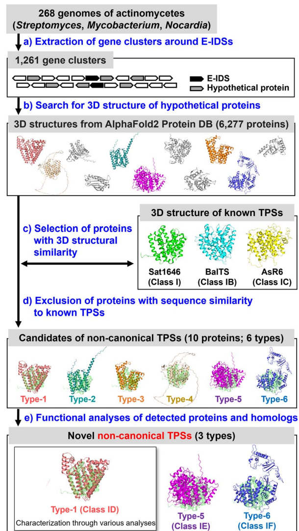
Fig. 1 Strategy for structural-model-based genome mining of non-canonical TPSs. Initially, 819 complete genomes of actinomycetes ( Streptomyces , Mycobacterium , and Nocardia ) published in ENA/DBJ/Genbank on 2023/06/12 were searched. However, 268 genomes for which the 3D structure models of the corresponding proteins were available from the AlphaFold DB were used. The workflow detected ten proteins (5, 4, and 1 proteins from Streptomyces , Mycobacterium , and Nocardia , respectively) as non-canonical TPS candidates and classified them into six types (types 1–6) based on their sequence similarities. (a–d) The 3D models of the candidates were superposed with the class I TPS (Sat1646, green structure). Functional analyses of each candidate type (e) revealed that three (1, 5, and 6) were new non-canonical TPSs (classes ID, IE, and IF). In this study, seven of the type-1 (class ID) homologs were also subjected to the functional analyses.
