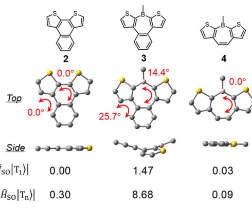
Fig. 8 DFT-optimized S 0 geometries of model compounds and their SOCMEs in cm -1 .
