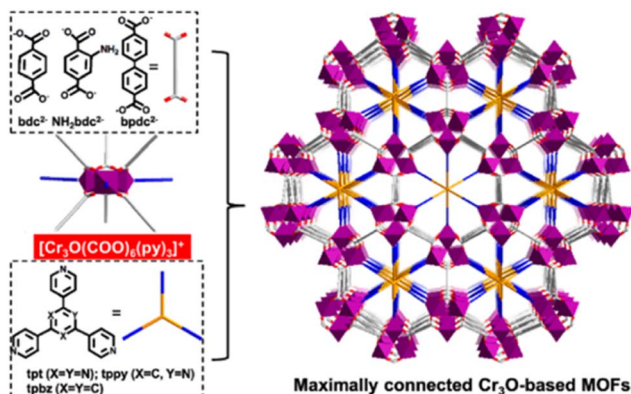
Fig. 13 The structural components, together with the framework viewed along the c axis. \text{NH}_2\text{bdc}^{2-} = 2-aminoterephthalate, \text{bpd}^{2-} = biphenyl-4,4'-dicarboxylate), \text{tpt} = 2,4,6-tri(4-pyridyl)-1,3,5-triazine (tpt), \text{tpbz} = 1,3,5-tri(4-pyridyl)-benzene, and \text{tppy} = 2,4,6-tris(4-pyridyl)pyridine. Reproduced from ref. 153 with permission from the American Chemical Society, Copyright 2021.
