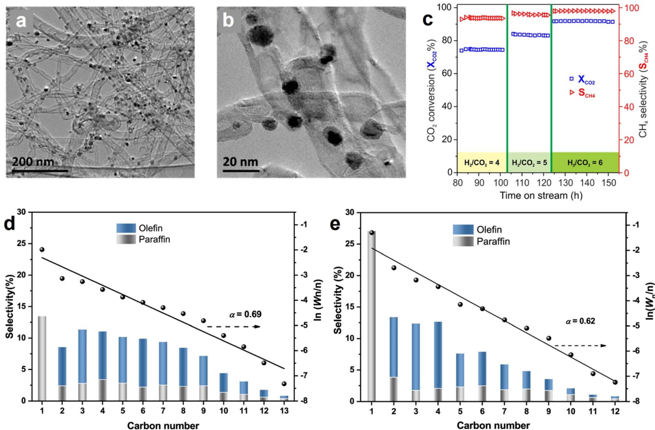
Fig. 12 (a and b) TEM images of Ni/N-CNT catalyst in different magnifications. (c) Influence of \text{H}_2/\text{CO}_2 ratio on the \text{CO}_2 methanation activity and selectivity Ni/N-CNT catalyst at a GHSV of 120\,000\text{ mL g}^{-1}\text{ h}^{-1} . Reproduced with permission from ref. 45. Copyright 2018, American Chemical Society. Hydrocarbon production distributions over the (d) FeK/SWNTs and (e) FeK/MWNTs catalysts after \text{CO}_2 hydrogenation test for 24 h. Reaction conditions: 0.2 g of catalyst, T = 613\text{ K} , P = 2.0\text{ MPa} , \text{H}_2/\text{CO}_2 = 3 , GHSV = 9000\text{ mL g}_{\text{cat}}^{-1}\text{ h}^{-1} . Anderson–Schulz–Flory (ASF) plots and \alpha -values (chain propagation probability) are also presented; W_n represents the weight fraction of a hydrocarbon with n carbon atoms. Reproduced with permission from ref. 169. Copyright 2021, American Chemical Society.
