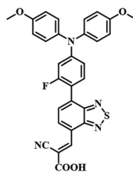
(28) MPA-BT-CA (PCE=21.24%)
