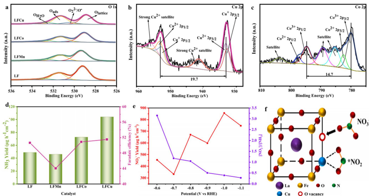
Fig. 15 (a–c) XPS spectra of O 1s, Cu 2p of LFCu, and Co 2p of LFCu. (d) Yield rate and Fes (NH 3 ) of the respective catalysts at -0.7 V (vs. RHE). (e) NO 2 - production and the ratio of [NO 2 - ] to [NH 3 ] on LFCu at various potentials, (f) schematic representation of NO 3 - reduction on LFCu. Reproduced from ref. 195 with permission from Elsevier, copyright 2023.
