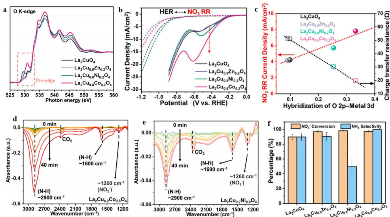
Fig. 16 O K-edge XAS spectra of the specified materials. (b) LSV curves for the La 2 CuO 4 , La 2 Cu 0.8 Co 0.2 O 4 , La 2 Cu 0.8 Ni 0.2 O 4 and La 2 Cu 0.8 Zn 0.2 O 4 . In 0.5 M Na 2 SO 4 solution in absence or presence of 2000 ppm nitrate. (c) Relationship of current density (NO 3 - reduction) vs. RHE, charge transfer resistance, and the O 2p-metal hybridization from the O K-edge XAS spectra. (d and e) In situ FT-IR analysis at -0.68 V vs. RHE for La 2 Cu 0.8 Co 0.2 O 4 and La 2 Cu 0.8 Ni 0.2 O 4 , respectively. (f) NH 3 selectivity and NO 3 - conversion. Reproduced with ref. 197 with permission from Elsevier, copyright 2022.
