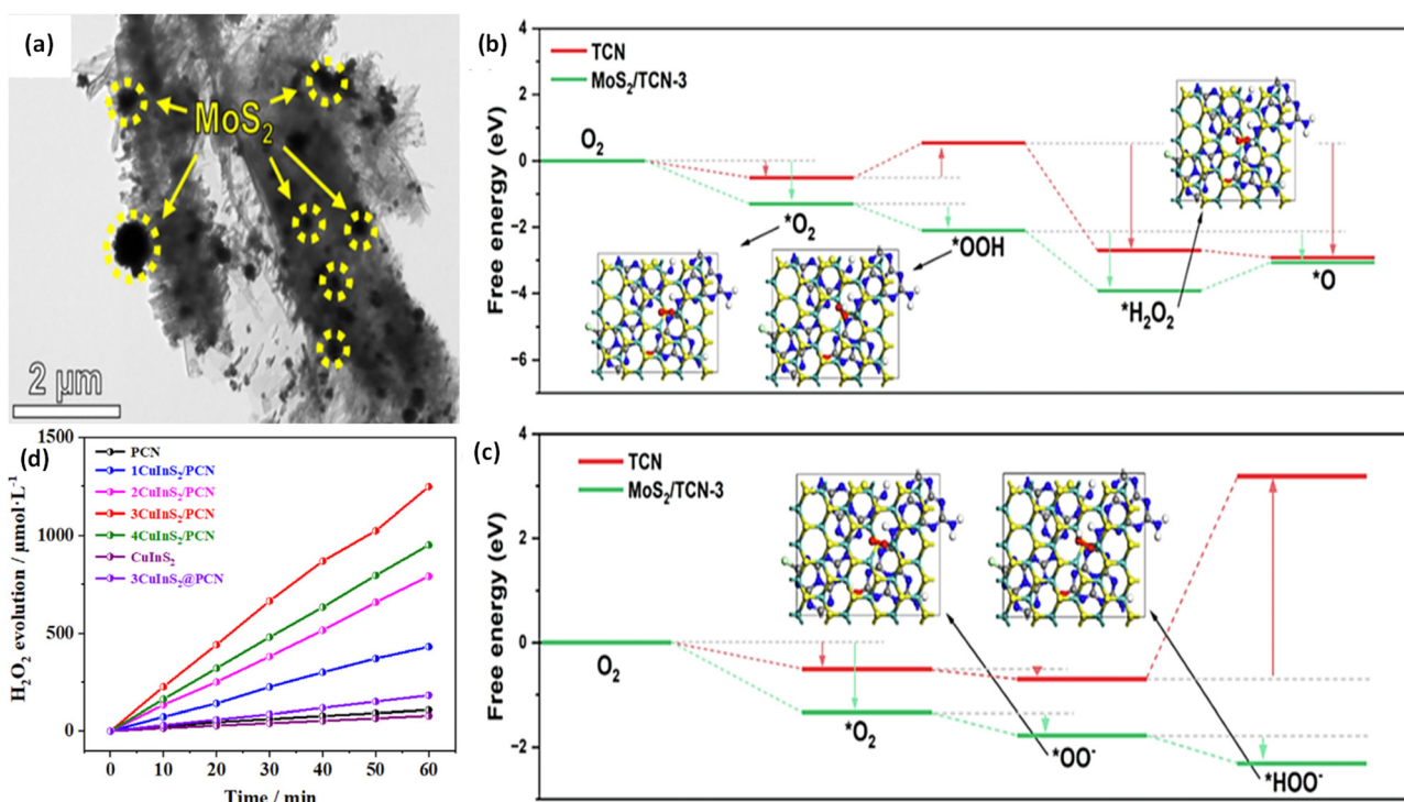
Fig. 27 (a) SEM images of \text{MoS}_2\text{-TCN-3} . Free energy change graphs for the \text{*HO}_2^- 2\text{e}^- ORR pathway under (b) acidic and (c) alkaline conditions. The figures are adapted with permission from ref. 201. Copyright 2023, Elsevier. (d) Photocatalytic \text{H}_2\text{O}_2 generation by PCN, \text{CuInS}_2 , 3\text{CuInS}_2@/\text{PCN} , and x\text{CuInS}_2/\text{PCN} samples. The figures are adapted with permission from ref. 202. Copyright 2023, Elsevier.
