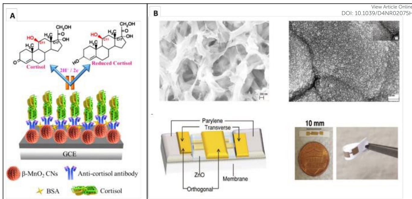
Fig. 8 A) Schematic representation of \text{MnO}_2 nanocacti electrochemical biosensor; 128 B) TEM pictures of the polyamide matrix before and after the deposition of ZnO, scheme of the electrochemical biosensor and real-life image of the biosensor. 129
