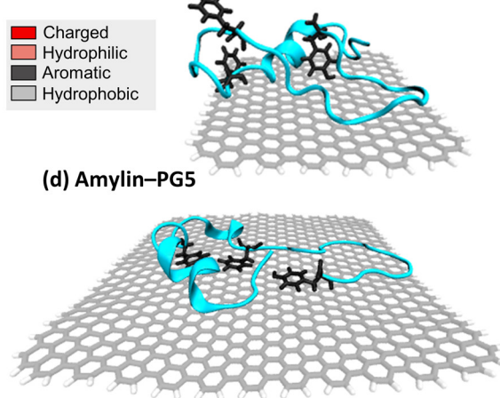
Fig. 2 Specific interactions between amylin and pristine graphene. (a) Average minimum distances measured between individual amylin residues and the PG3, PG5, and PG7 surfaces. Calculated on the lowest energy states of each system (shown in Fig. 1), with errorbars representing standard deviation. Shaded grey on the plot is used to indicate residue–NF contacts, defined as distances less than 0.4 nm. Residue numbers are coloured by sidechain physicochemical properties: dark red – charged (Lys and Arg); light red – hydrophilic (Asn, Thr, Gln, His, Ser and Cys); light grey – hydrophobic (Ala, Leu, Val, Gly and Ile); and dark grey – aromatic (Phe and Tyr). (b)–(d). Representative snapshots that highlight favourable amylin–PG interactions. The amylin backbone is shown in cyan cartoon representation, residue sidechains are drawn in licorice atomic detail and coloured based on their properties ( i.e. , charged, hydrophilic, hydrophobic, and aromatic), and graphene carbon atoms are shown in grey with either space-filling (b) or licorice (c and d) representations. Water and ions are hidden for clarity. (b) Top-view of amylin–PG5 showing residues within 0.4 nm of the NF. (c), (d). Side-view of amylin interacting with PG3 and PG5, emphasising the orientation of aromatic residues relative to the substrates.
