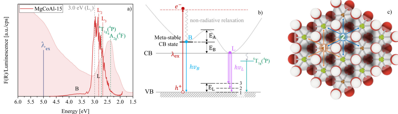
Fig. 2 (a) Comparison of the absorption and luminescence spectrum of MgCoAl-15 at 298 K. The position of the two spin-allowed d–d transitions {}^4T_{1g}({}^4P) and {}^4A_{2g}({}^4F) is indicated in green, while the position of the bandgap (3.0 eV overlapping with L_1 ) is depicted in grey and the positions of L_2 and L_3 are depicted in red. \lambda_{ex} = 5.0 eV. (b) Depiction of the expected radiative transition pathways to create the luminescence bands B and L. E_A is the activation energy required to overcome entrapment in the meta-stable CB band, which minimum is located E_B above the CB edge. E_L describes the highest energy state above the VB edge involved to create the triple-sub-band feature of band L. The path through {}^4T_{1g}({}^4P) is depicted for illustrative purposes. (c) Depiction of a 2 : 1 LDH lattice with perfect ordering of Mg^{2+} and Al^{3+} ions in the lattice replaced with (1) a Co^{3+} ion (nearest neighbours Mg or Co cations) and (2) a Co^{2+} ion (nearest neighbours Al, Mg or Co cations). The likelihood of a Co-nearest-neighbour increases with Co-content.
