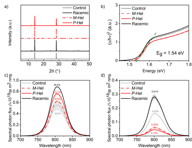
Fig. 2 Effect of helical modulation on the properties of \text{FA}_{0.97}\text{MA}_{0.03}\text{Pb}(\text{I}_{0.97}\text{Br}_{0.03})_3 perovskite films. (a) XRD patterns and (b) the corresponding T_{\text{auc}} plots. (c and d) Absolute intensity steady-state PL for control (grey) and modulated (red, black) films on microscope glass in the absence (c) and presence (d) of HTM (spiro-OMeTAD). Numbers represent PLQY and quasi-Fermi level splitting ( \Delta E_{\text{F}} ; Table S6†). 40 TRPL data is shown in Fig. S19–S21†
