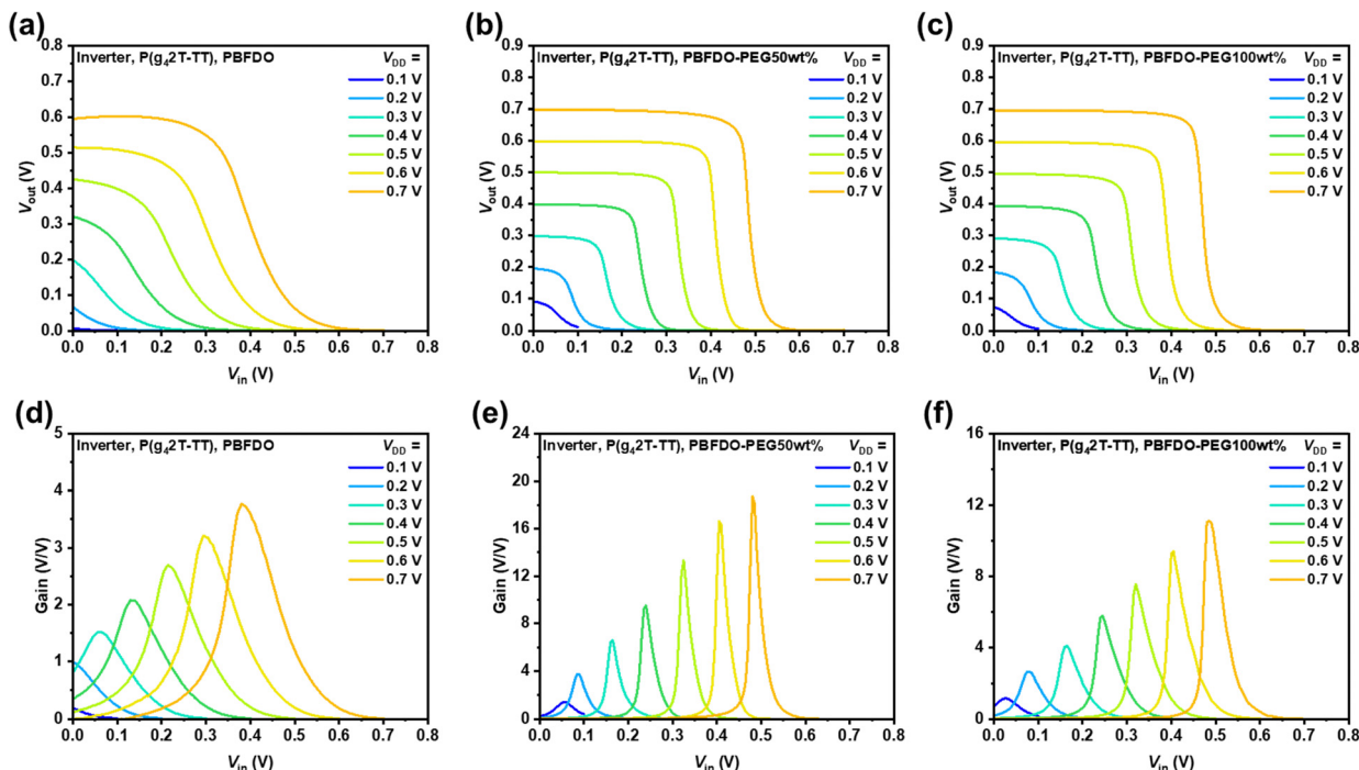
Fig. 6 OECTs-based complementary inverters. The voltage transfer characteristics and gain of inverters based on P(g_42T-TT) with different n-type channel materials (a) and (d) PBFD0, (b) and (e) PBFD0-PEG50wt%, (c) and (f) PBFD0-PEG100wt%.
