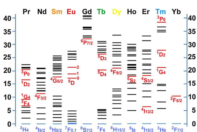
Fig. 5 Partial energy diagrams for the lanthanide aqua ions; the values of the energy levels are given as 1000 \text{ cm}^{-1} . The red and blue lines indicate the main luminescence and the fundamental levels, respectively. Reprinted with permission from Elsevier. 57
