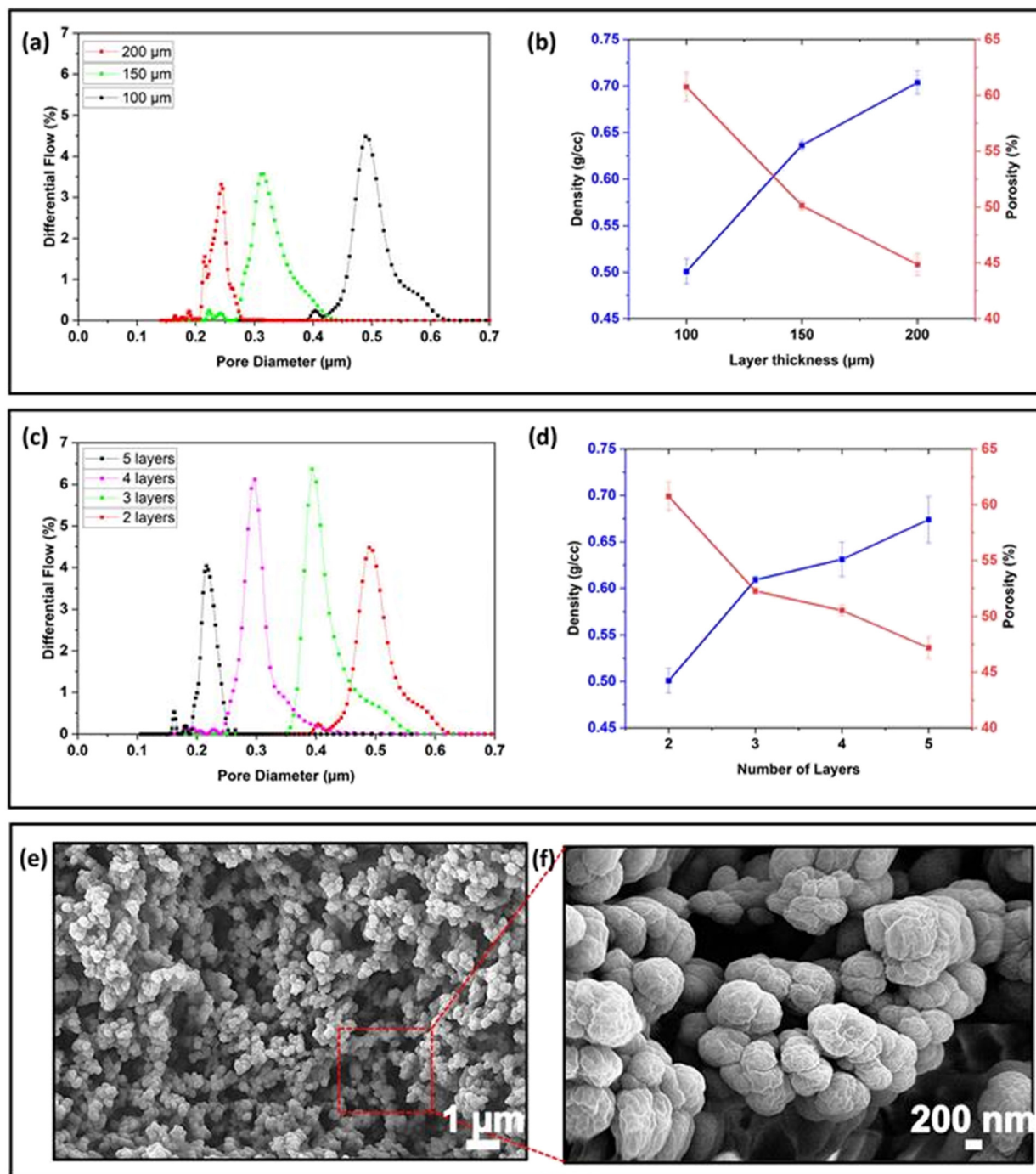
Fig. 3 (a) Average pore size/distribution and (b) porosity/density under the different layer thicknesses. (c) Average pore size/distribution and (d) porosity/density under the different layer numbers. (e and f) SEM images of the porous structure of the membrane under the optimal printing conditions.
