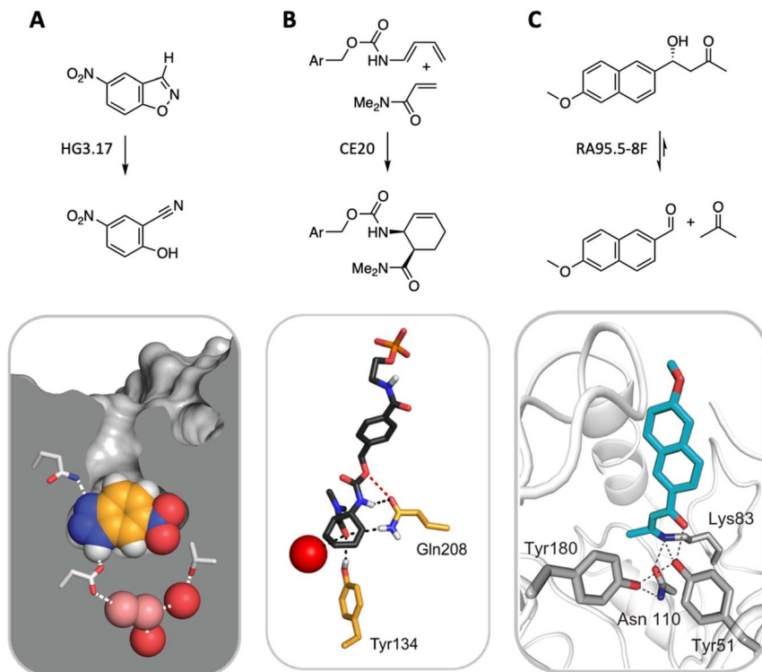
Fig. 6 Three representative examples of computationally designed enzymes that have been evolved to high activity and selectivity by iterative rounds of mutagenesis and screening. (A) A Kemp eliminase for proton transfer from carbon, 62 (B) a stereospecific Diels–Alderase, 65 and (C) a multi-step aldolase that exploits amine catalysis. 68
