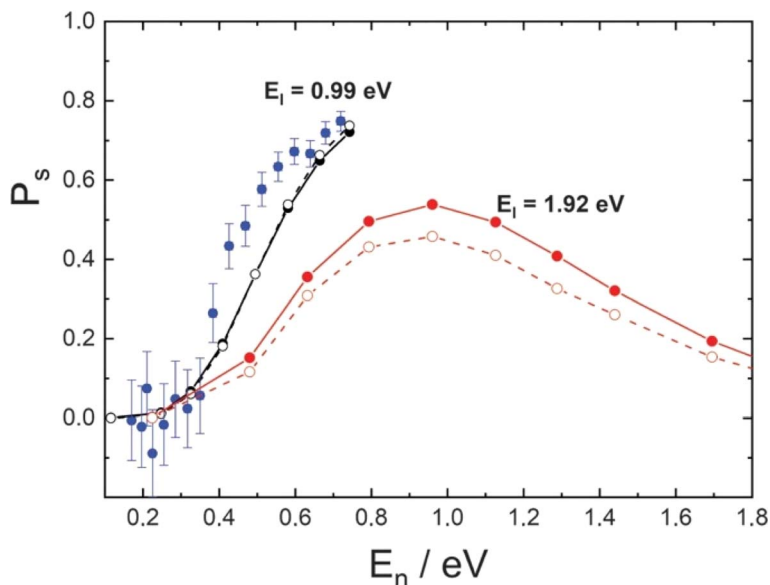
Fig. 9 H-atom sticking probabilities at graphene. Experimentally derived (blue) and theoretically predicted (black) sticking probabilities for E_i = 0.99 \text{ eV} plotted against the normal component of the incidence energy ( E_n ). Theoretically predicted sticking probabilities for E_i = 1.92 \text{ eV} are shown in red. Theoretical simulations used a full-dimensional EMFT-REBO PES that includes the influence of the Pt substrate with classical molecular dynamics (solid symbols) or ring polymer molecular dynamics (open symbols). Adapted from ref. 360 and used with permission under lic. no. 5743000308890.
