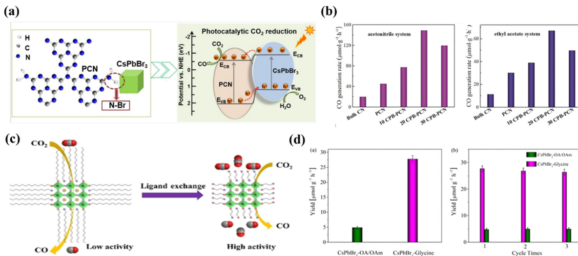
Fig. 13 (a) CsPbBr 3 QDs were anchored on the porous semiconductor g-C 3 N 4 porous nanosheets via strong N-Br bonds. 111 (b) Generation of CO in the acetonitrile/water (left) and ethyl acetate/water system (right) over various photocatalysts. 111 (c) Glycine-functionalized CsPbBr 3 nanocrystals are constructed through a facile ligand-exchange strategy. 112 (d) Yields of CO generated from CO 2 reduction with CsPbBr 3 -OA/OAm and CsPbBr 3 -glycine NCs as photocatalysts, under Xe-lamp irradiation for 4 h with a 400 nm filter and a light intensity of 100 mW cm -2 (left) and yields of CO generated from CO 2 reduction for three consecutive cycles of 4 h each with CsPbBr 3 -OA/OAm and CsPbBr 3 -glycine NCs as photocatalysts (right). 112
