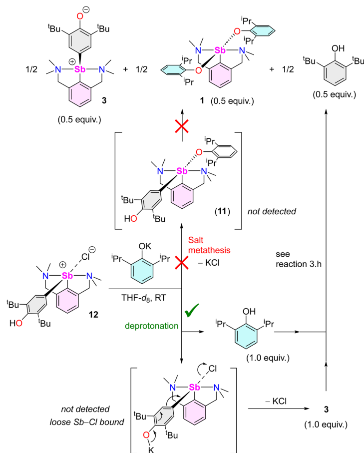
Scheme 5 Reaction of [\{\text{NCN}^{\text{Me}_4}\}\text{Sb}(\text{C}_6\text{H}_2\text{-}^t\text{Bu}_2\text{-3,5-OH-4})\text{Cl}]\text{Cl} ( 12 ) with [\{2,6\text{-}i\text{Pr}_2\text{-C}_6\text{H}_3\text{O}\}]\text{K} , highlighting the two potential mechanistic pathways.
