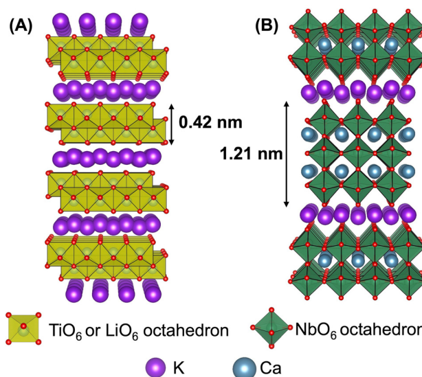
Fig. 30 Crystal structures of (A) lepidocrocite-type layered titanate K_{0.8}Ti_{1.73}Li_{0.27}O_4 and (B) Dion–Jacobson-type layered perovskite KCa_2Nb_3O_{10} . The structural parameters were referred from ref. 528 and 529, respectively. The crystal structure was drawn using the VESTA program. 44
