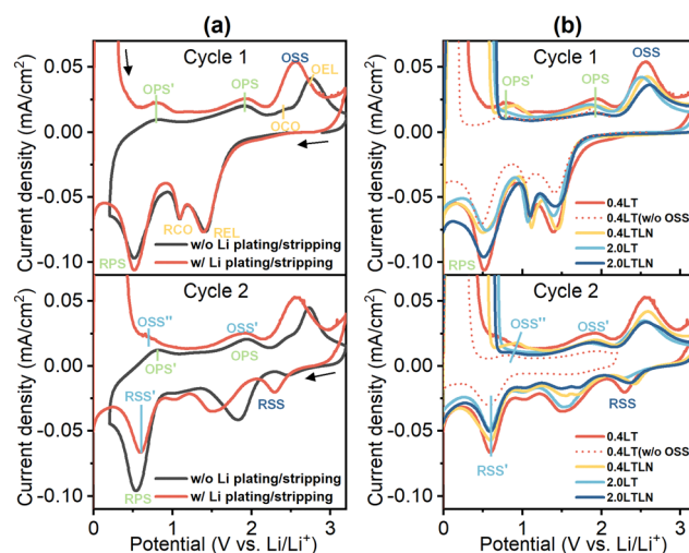
Fig. 1 (a) Enlarged view of the first- and second-cycle CV curves measured in 0.4LT; (b) enlarged view of the first- and second-cycle CV curves measured in 0.4LT, 0.4LT w/o OSS, 0.4LTN, 2.0LT and 2.0LTN with Li plating/stripping. The prime symbols ' and '' on the capitals indicate that the corresponding peaks locate at a lower potential compared to those without the prime symbol. The arrows represent the direction of scanning. Potential range with Li plating/stripping: -0.5 to 3.2 V, and potential range w/o Li plating/stripping: 0.2 – 3.2 V. Scan rate: 10 \text{mV s}^{-1} .
