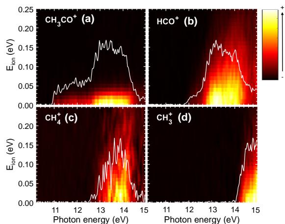
Fig. 5 Ion signal correlated to threshold photoelectrons as a function of ion kinetic energy, E_{ion} and photon energy. The photon energy axis corresponds to the ionization energy since only threshold electrons are considered. The TPES obtained for CoM-KER below 25 meV is plotted as white curves. The color bar on the right represents the intensity (in arb. units).
