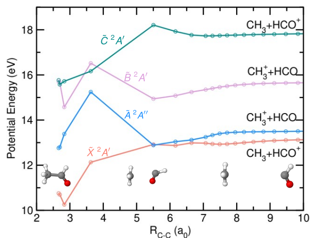
Fig. 10 Potential energy of the first four electronic states of CH 3 CHO + , \tilde{X}^2A' , \tilde{A}^2A'' , \tilde{B}^2A' and \tilde{C}^2A' , as a function of the C–C bond distance (in atomic units, a 0 ) resulting from the NEB calculations, optimized for the formation of CH 3 + and HCO. Relevant geometries, i.e. at the Franck-Condon region, at R C-C = 5.5 a 0 and at the asymptotic limit, are also drawn. The two first dissociation limits correspond to the formation of the two fragments in their respective ground electronic states while the third and the fourth correspond to the formation of HCO and HCO + , in their respective first excited electronic states.
