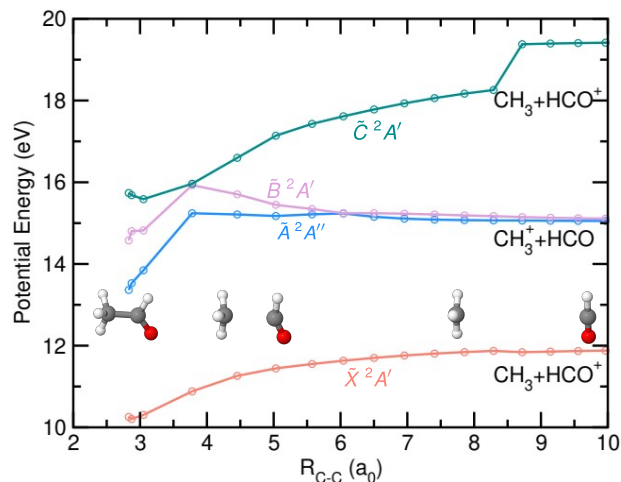
Fig. 9 Potential energy of the first four electronic states of CH 3 CHO + , \tilde{X}^2A' , \tilde{A}^2A'' , \tilde{B}^2A' and \tilde{C}^2A' , as a function of the C–C bond distance (in atomic units, a 0 ) resulting from the NEB calculations optimized for the formation of CH 3 and HCO + . Relevant geometries, i.e. at the Franck-Condon region, at R C-C = 4.45 a 0 and at the asymptotic limit, are also drawn. The two first dissociation limits correspond to the formation of the two fragments in their respective ground electronic states while the third corresponds to the formation of HCO + in its first excited electronic state.
