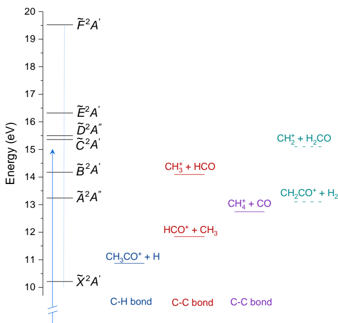
Fig. 1 Schematic energy diagram showing the cationic electronic states of acetaldehyde (left) and the different fragmentation pathways. Blue arrow represents one-photon ionization at h\nu=15 eV (results in Fig. 3 and the blue square indicate the energy region of the threshold photoelectron spectrum (TPES, Fig. 4). The two additional fragmentation pathways reported here are shown in dashed lines.
