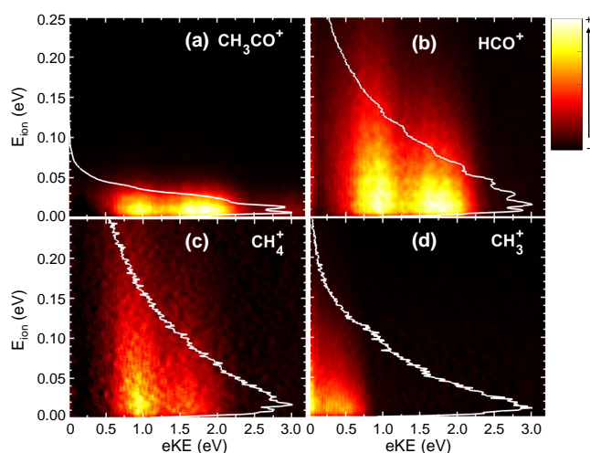
Fig. 3 Electron-ion kinetic energy correlation diagrams, photoelectron energy (eKE) vs. photoion kinetic energy ( E_{ion} ), at photon energy of 15.0 eV for (a) CH 3 CO + , (b) HCO + , (c) CH 4 + , and (d) CH 3 + . The color bar on the right represents the intensity (in arb. units). The corresponding E_{ion} distributions are depicted as white lines.
