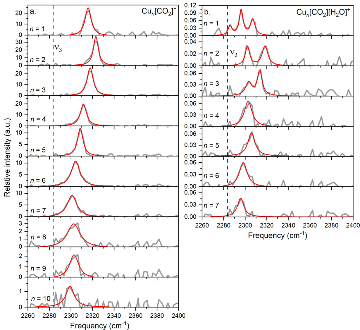
Fig. 2 (a) The average of experimental photodissociation spectra of the \text{Cu}_n[\text{CO}_2]^+ complexes, covering the range of n = 1 – 10 , within the vibration spectrum of the \text{CO}_2 asymmetric stretch, is showcased in grey. (b) The same spectral range investigated for \text{Cu}_n[\text{CO}_2][\text{H}_2\text{O}]^+ complexes, n = 1 – 7 . On both graphs, the Lorentzian-fitted bands are highlighted in red. Additionally, the position of the band determined for free \text{CO}_2 is indicated with a dashed line.
