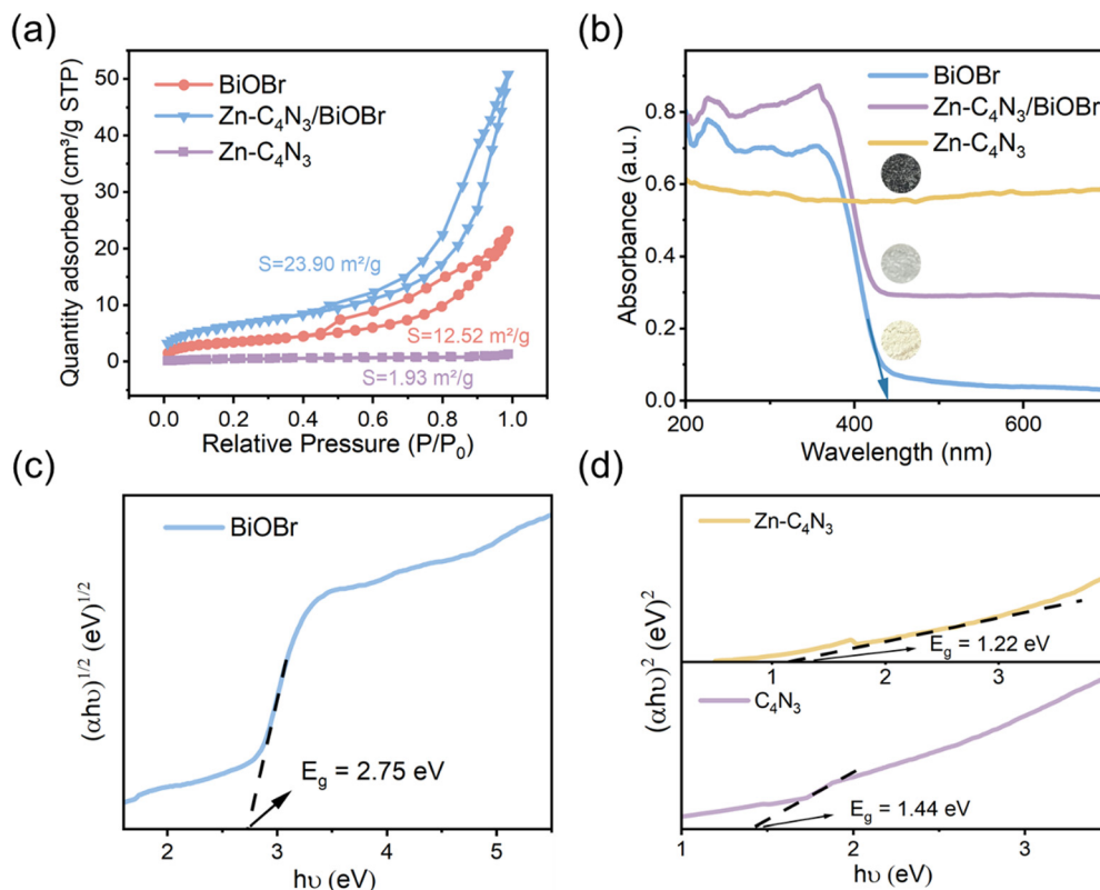
Fig. 3 (a) N 2 adsorption–desorption isotherms of BiOBr and Zn– C_4N_3 /BiOBr. (b) UV-vis absorption spectra of the different catalysts (inset: digital pictures of photocatalysts). (c) and (d) The band gaps of BiOBr, C_4N_3 and Zn– C_4N_3 .
