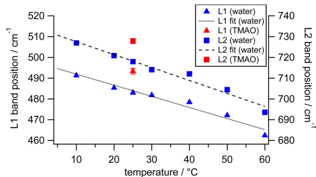
Fig. 6 The peak positions of the librational L1 bands (triangles) and the librational L2 bands (squares) originating from water in the HR spectra of water (blue) and the TMAO aqueous solution at 0.5 M (red) at different temperatures. Black dashed lines are the fits of the librational band positions.
