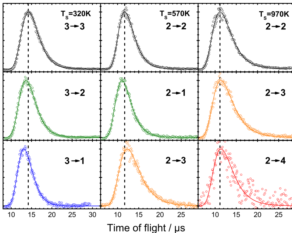
Fig. 17 Example of experiments where laser-prepared NO ( v_i, J_i ) with well-defined translational energy of incidence collides with a Au(111) surface within a narrow arrival time window. The resulting (quantum-state-resolved) NO ( v_f, J_f ) time-of-flight traces indicating the time it takes to recoil from the surface to the (REMPI) detector are recorded. The vertical dashed lines are drawn to the peaks of the time-of-flight distributions of the elastic channels to illustrate the small differences for the vibrationally inelastic channels. The data cover vibrationally elastic scattering (black) as well as loss of one (green) and two (blue) quanta and gain of one (orange) and two (red) quanta of molecular vibration. From ref. 39 with permission from American Chemical Society, Copyright (2013).
