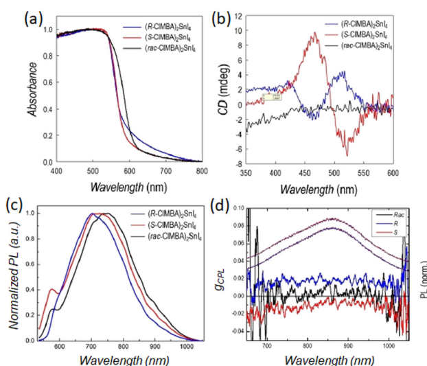
Fig. 24 (a) Absorbance; (b) CD, and (c) \mu\text{PL} spectra of (R/S\text{-}Rac\text{-}CIMBA)_2\text{SnI}_4 . (d) g_{CPL} (left axis) and static PL (right axis) for (R/S\text{-}Rac\text{-}CIMBA)_2\text{SnI}_4 measured at 90 K. Reprinted with permission from ref. 43 Copyright©2024 Wiley-VCH GmbH.
