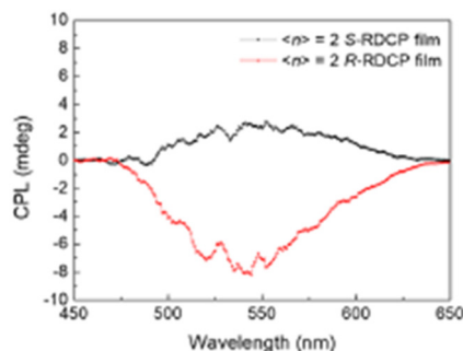
Fig. 27 CPL spectra of (R/S-Rac-MBA) 2 (CsMA)Pb 2 Br 7 . Reprinted with permission from ref. 47 Copyright©2022 American Chemical Society.
