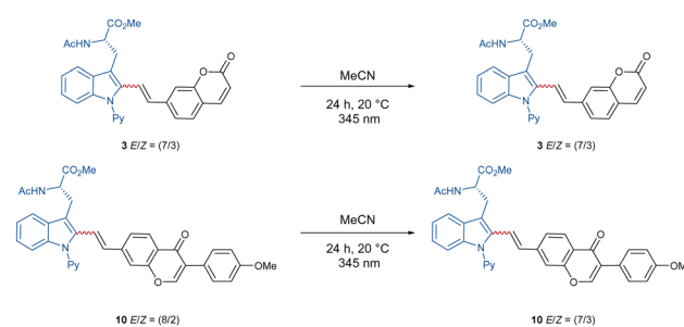
Scheme 3 Isomerization studies.
