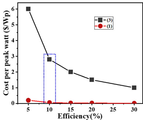
Fig. 7 Cost per peak watt ($ per Wp) for (1) and spiro-OMeTAD (3).
