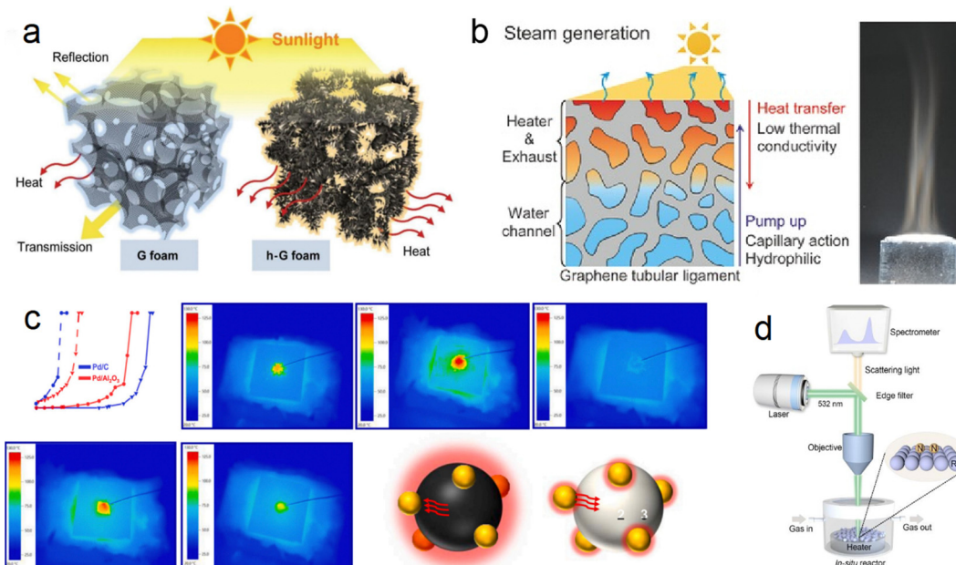
Fig. 5 (a) Difference in solar-thermal conversion processes between ordinary graphene foam and hierarchical graphene foam. 64 (b) Multifunctional nanoporous graphene converting solar illumination into high-energy steam. 65 (c) Heat transfer path in CO conversion proved by IR monitoring images (carbon support \rightarrow Pd \rightarrow \text{Al}_2\text{O}_3 ). 66 (d) Schematic illustration of the customized in situ Raman system. 67
