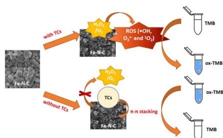
Scheme 1 Schematic illustration of the colorimetric biosensor for TCs detection using Fe–N–C as a nanozyme.
