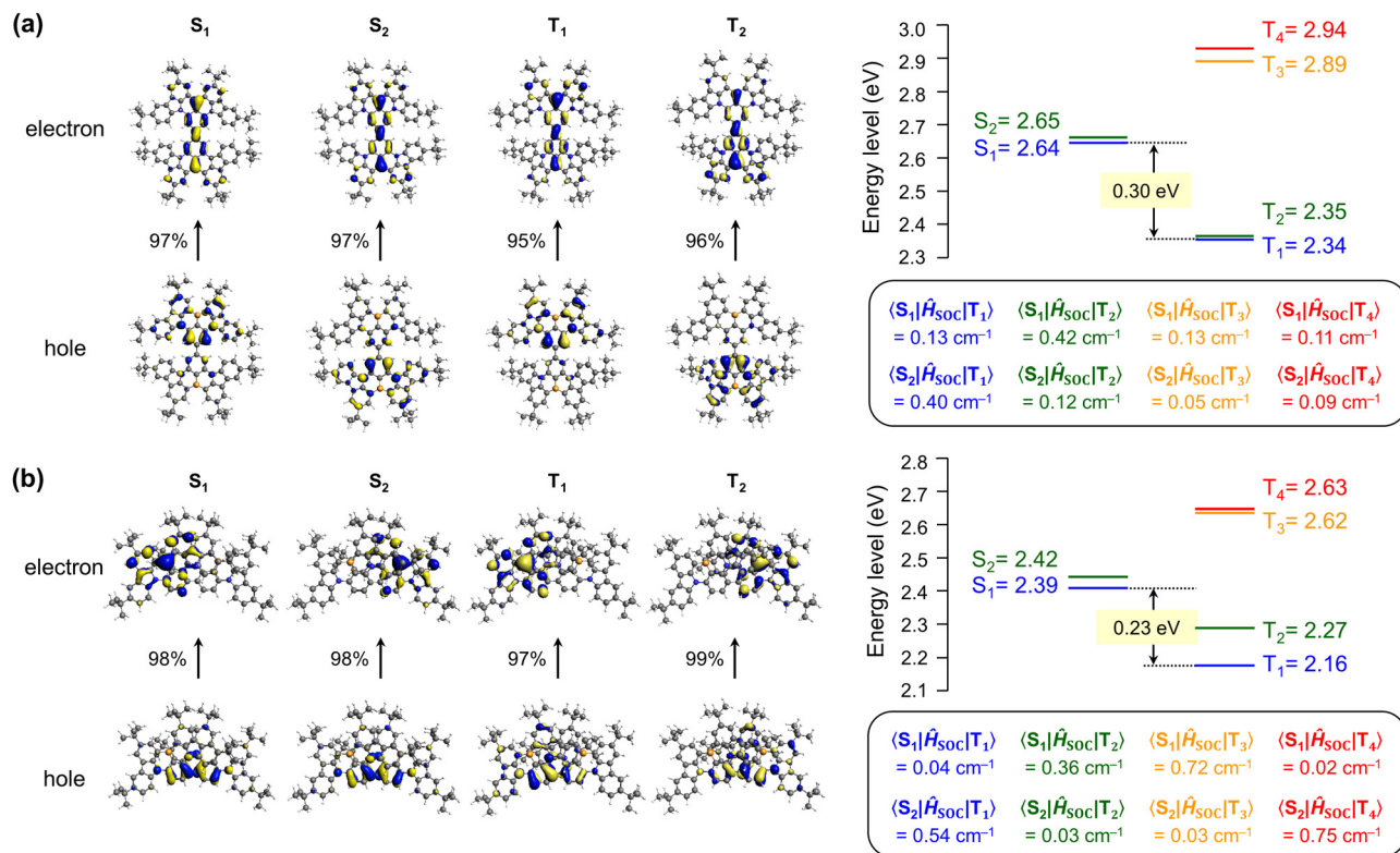
Fig. 3 Natural transition orbitals (NTOs) for the excited singlet ( S_m ) and triplet ( T_n ) states and simulated energy-level diagrams for (a) p-CzB and (b) m-CzB . NTOs, excitation energies for S_m and T_n , and associated spin–orbit coupling (SOC) matrix elements between the T_n and S_m states were calculated at the B3LYP/DZP level.
