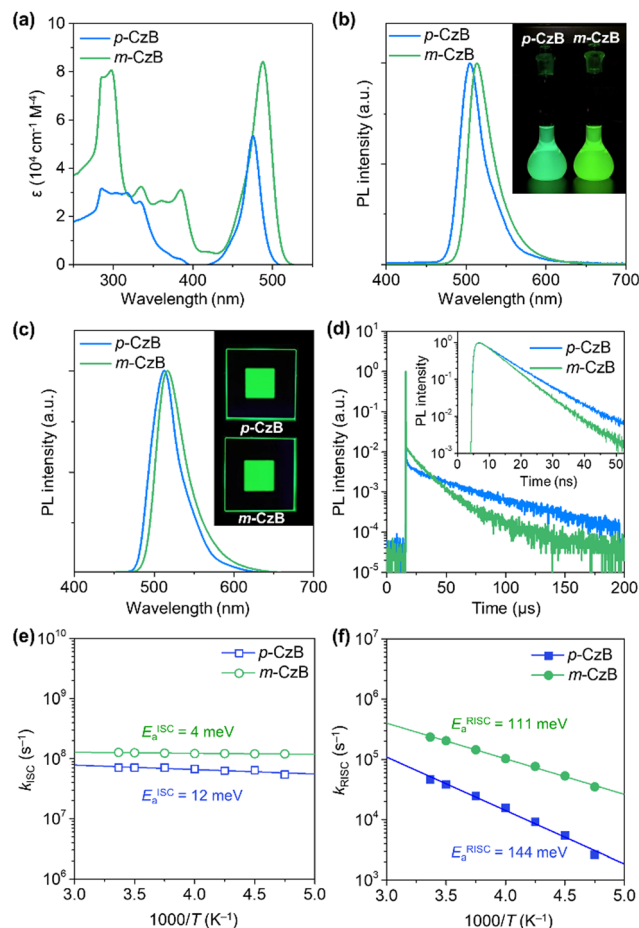
Fig. 2 (a) UV-vis absorption and (b) PL spectra of p-CzB and m-CzB in deoxygenated toluene ( 10^{-5} M) with a photographic image showing green emissions when illuminated by UV light (365 nm). (c) Steady-state PL spectra with corresponding emission images and (d) transient PL decay profiles acquired at 300 K for the doped films of p-CzB and m-CzB in mCBP-CN host matrices at a doping concentration of 1 wt%. The inset in (d) shows transient PL in the nanosecond (0–50 ns) region. (e and f) Arrhenius plots of k_{\text{ISC}} and k_{\text{RISC}} measured with the 1 wt%-emitter: mCBP-CN doped films, in which the solid lines represent the least-squares fittings for determining E_{\text{a}}^{\text{ISC}} and E_{\text{a}}^{\text{RISC}} .
