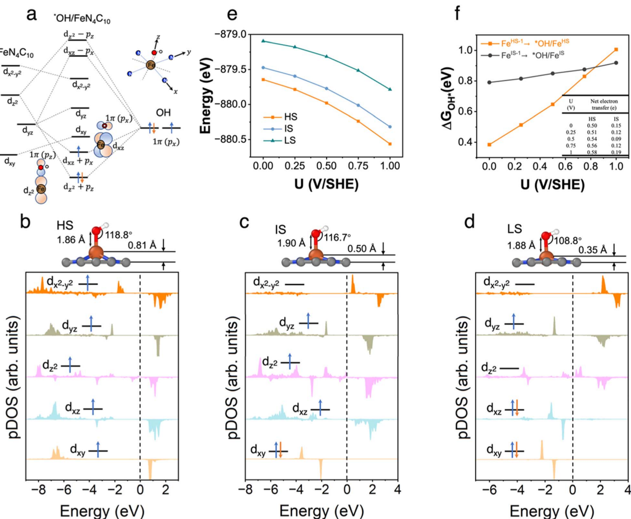
Fig. 5 ^*\text{OH}/\text{FeN}_4\text{C}_{10} . (a) Schematics of orbital hybridizations of Fe 3d orbitals in a square-planar ligand field with the 2p orbitals in the OH adsorbate. (b)–(d) Atomic structures and pDOS plots of the HS, IS, and LS states of ^*\text{OH}/\text{FeN}_4\text{C}_{10} . (e) Spin- and potential-dependent energies of ^*\text{OH}/\text{FeN}_4\text{C}_{10} under constant-potential conditions. (f) Spin and potential-dependent ^*\text{OH} adsorption energies. The inset table shows the net electron transfer in the adsorption process.
