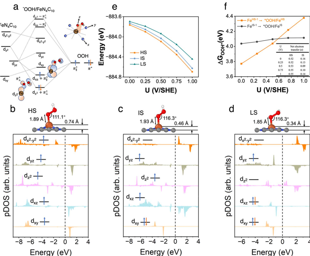
Fig. 3 *OOH/FeN 4 C 10 . (a) Schematics of orbital hybridization of Fe 3d orbitals in a square-planar ligand field with the molecular orbitals in the OOH adsorbate. (b)–(d) Atomic structures and pDOS plots of the HS, IS, and LS spin states of *OOH/FeN 4 C 10 . (e) Spin- and potential-dependent energies of *OOH/FeN 4 C 10 under constant-potential conditions. (f) Spin and potential-dependent *OOH adsorption energies. The inset table shows the net electron transfer in the adsorption process.
