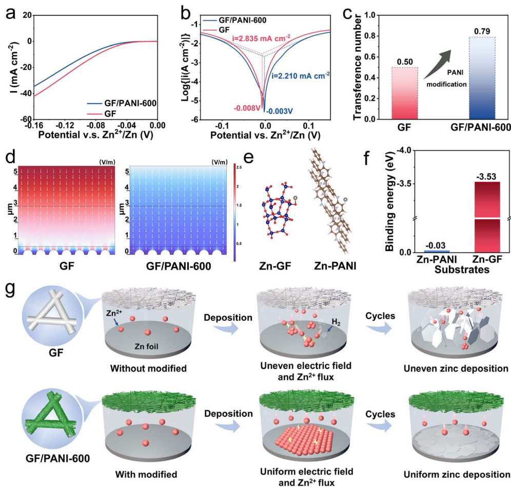
Fig. 4 (a) LSV curves at a scan rate of 5.0 mV s -1 and (b) Tafel plots of the Zn||Zn symmetric batteries with different separators. (c) The calculated transference number of zinc ions ( t Zn 2+ ). (d) The electrical field distribution on the GF and GF/PANI-600 separators. (e) Optimized adsorption configurations and (f) the corresponding binding energy of GF and PANI-600 with Zn. (g) The schematic demonstration of the evolution of the plating process on Zn anodes with GF/PANI-600 and pristine GF separators.
