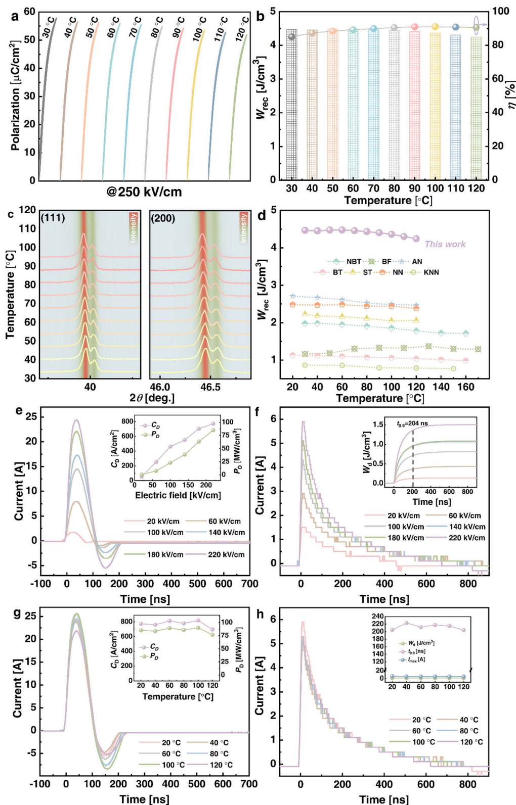
Fig. 7 (a) Unipolar P - E loops (measured at 250 kV cm ^{-1} ) and (b) W_{\text{rec}} and \eta as functions of temperature for x = 0.08 (VPP) ceramics. (c) Temperature evolution of XRD patterns for x = 0.08 (VPP) ceramics from 30 °C to 120 °C at selected angles of 39.5–40.5° and 46–47°. (d) Comparison of W_{\text{rec}} at temperatures between this work and some recently reported lead-free ceramics. (e) Underdamped discharge and (f) overdamped discharge waveforms of the x = 0.08 (VPP) ceramic under various electric fields and ambient temperature. (g) Underdamped discharge and (h) overdamped discharge waveforms of the x = 0.08 (VPP) ceramic measured in the temperature range from 20 to 120 °C under 220 kV cm ^{-1} .
