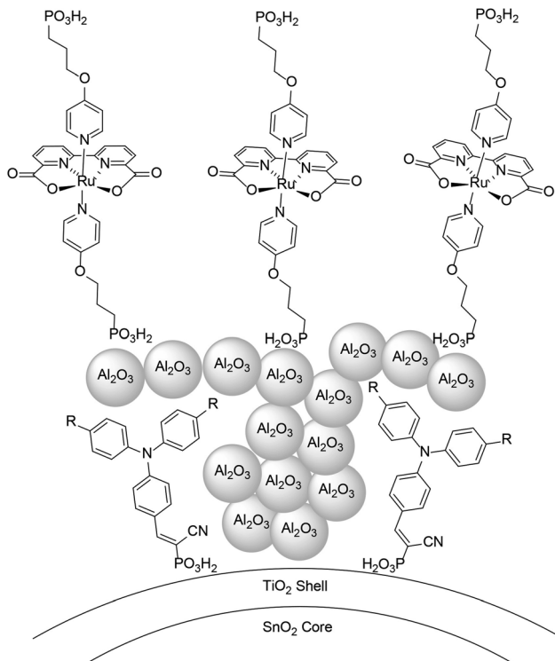
Fig. 22 4.5 nm SnO 2 /TiO 2 particles sensitized with a triphenylamine photosensitizer, embedding a 7–10 Å Al 2 O 3 protecting layer, exploited to anchor a Ru(bda) WOC. Reprinted from ref. 127 with permission from the American Chemical Society, copyright 2017.
