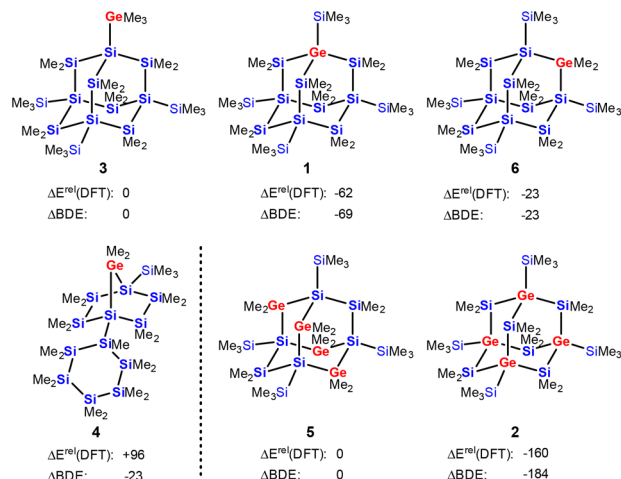
Fig. 3 Relative energies \Delta E^{\text{rel}} (DFT), in kJ mol -1 , of selected \text{Si}_{13}\text{Ge}_1\text{-Me}_{24} and \text{Si}_{10}\text{Ge}_4\text{Me}_{24} isomers. Both calculated at M06-2X/6-311+G(d,p) and estimated on the basis of bond dissociation energies \Delta \text{BDE} .
