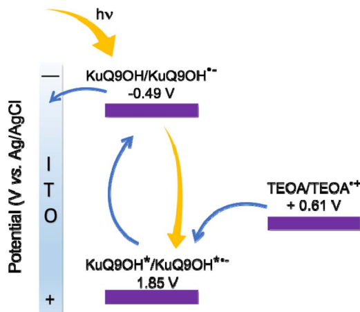
Fig. 8 Proposed mechanism for anodic photocurrent generation of \text{KuQ9OH|ITO/H}_2\text{O/Na}_2\text{SO}_4 0.1 M/TEOA 50 mM.
