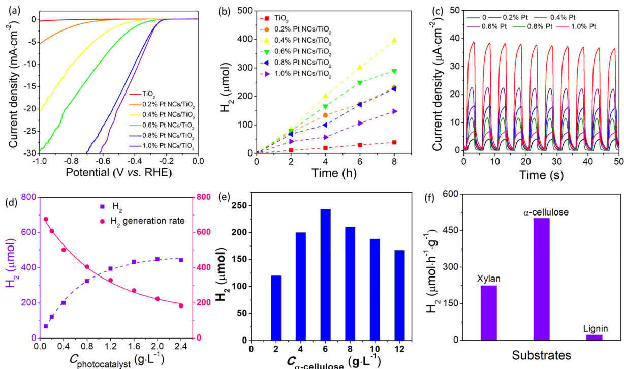
Fig. 3 (a) LSV plots of bare \text{TiO}_2 and various Pt/ \text{TiO}_2 electrodes. (b) Time course of photocatalytic \text{H}_2 production over various Pt/ \text{TiO}_2 photocatalysts in \alpha -cellulose aqueous solution. (c) Photocurrent density of bare \text{TiO}_2 and various Pt/ \text{TiO}_2 electrodes. (d) Photocatalytic \text{H}_2 yields as a function of photocatalyst concentration in \alpha -cellulose aqueous solution, irradiation time 4 h. (e) Photocatalytic \text{H}_2 yields as a function of \alpha -cellulose concentration using 0.4% Pt/ \text{TiO}_2 as a photocatalyst, irradiation time 4 h. (f) Photocatalytic \text{H}_2 generation rate of 0.4% Pt/ \text{TiO}_2 in \alpha -cellulose, xylan and lignin aqueous solutions. Photocatalytic reaction conditions: 100 mg photocatalyst, 300 W Xe lamp, 1 g substrate, and 250 ml water.
