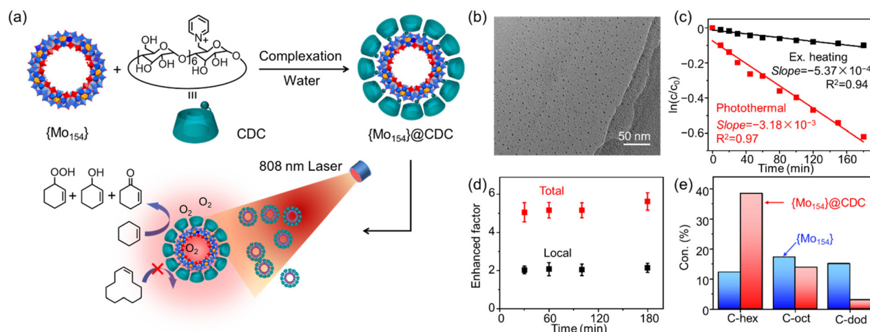
Fig. 8 (a) Schematic illustration for the complex comprising of \{\text{Mo}_{154}\} and CDC, and its photothermal catalysis for the oxidation of olefins under irradiation with an 808 nm laser. (b) TEM image of \{\text{Mo}_{154}\}@ CDC at 65 °C. (c) Catalytic kinetic curves of the substrate cyclohexene catalyzed by \{\text{Mo}_{154}\}@ CDC versus the reaction time under different temperature conditions. (d) The calculated enhanced factors of \text{Con. (P.T.)} / \text{Con. (R.T.)} in the black square versus the reaction time. (e) Conversions of the oxidation of a series of alkenes (C-hex, cyclohexene; C-oct, cyclooctene; C-dod, and cyclododecene) over the catalyst \{\text{Mo}_{154}\}@ CDC and the isolated \text{Na}_{14}\{\text{Mo}_{154}\} cluster. Reproduced from ref. 100. Copyright 2021, AAAS.
